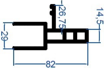
E-1709 1,356 kg/m
